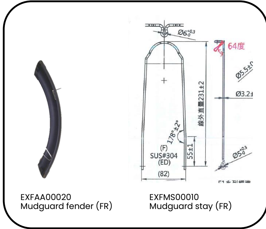
EXFMA00020 Front Mudguard Kit
